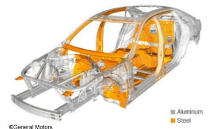
CADILLAC CT6 MIXED-MATERIAL STRUCTURE
